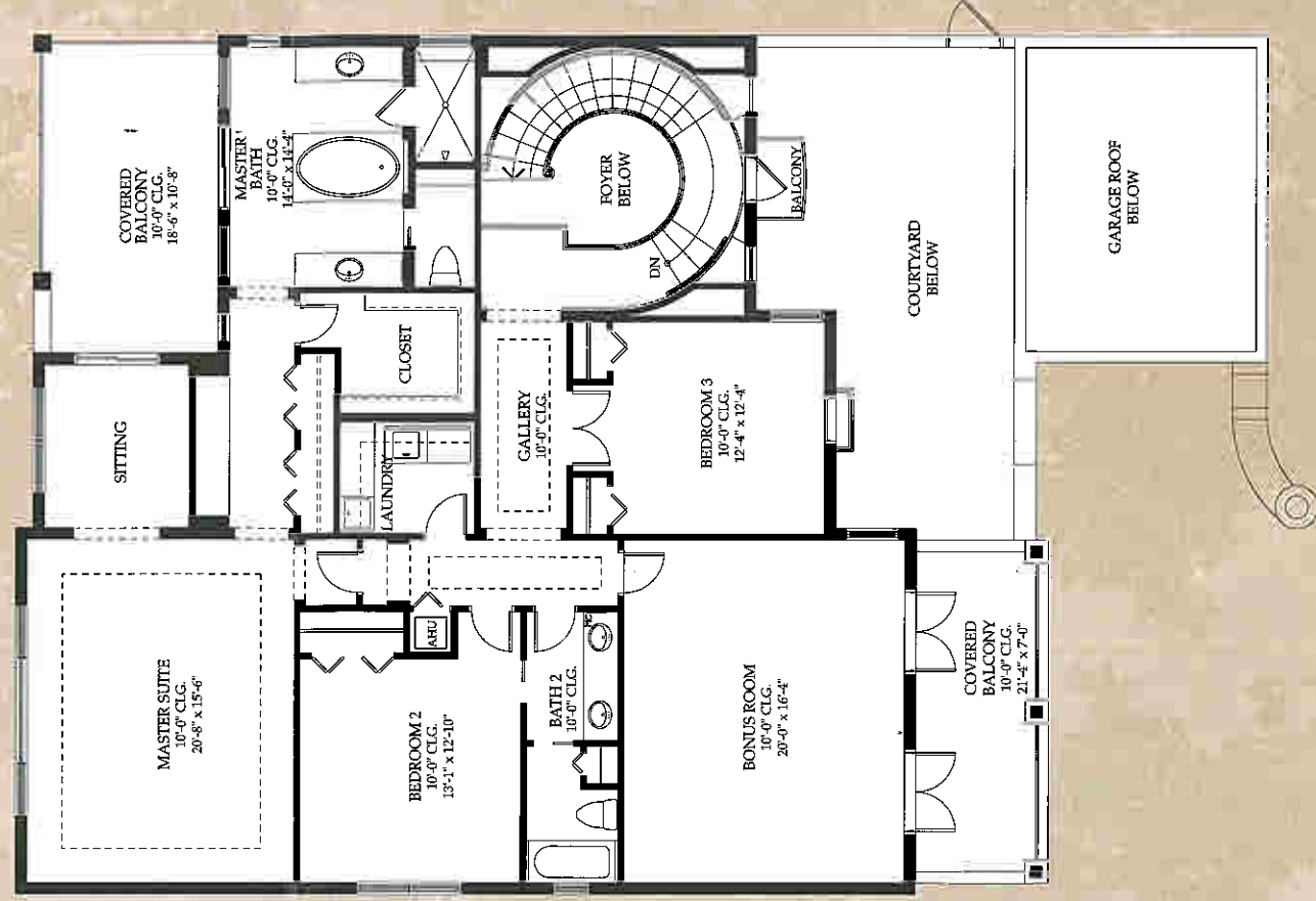
SECOND FLOOR
